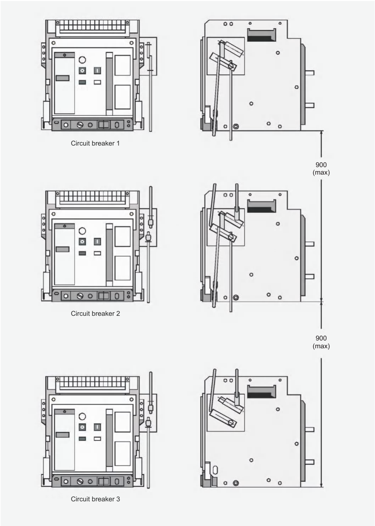
Figure 13 Interlocking with connecting rods for the stacked circuit breaker
