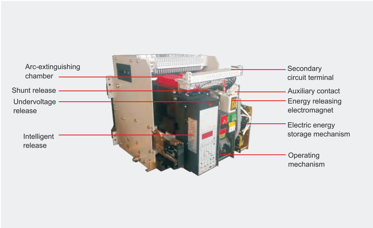
Figure 6. Extraction position of the KNW1 Series Universal Circuit Breaker
