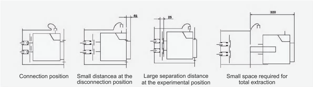
Figure 8. The circuit breaker is small in size and compact in structure, and only a small space is needed for buttons and operations. It has good safety at the "test" or "disconnection" position.
