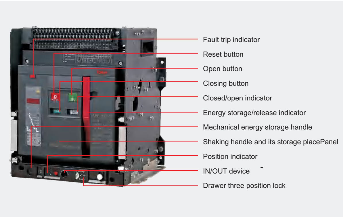
Figure 5. Operation indicator diagram of the KNW1 Series Universal Circuit Breaker
