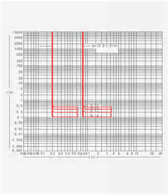
Figure 2. Grounding fault protection
