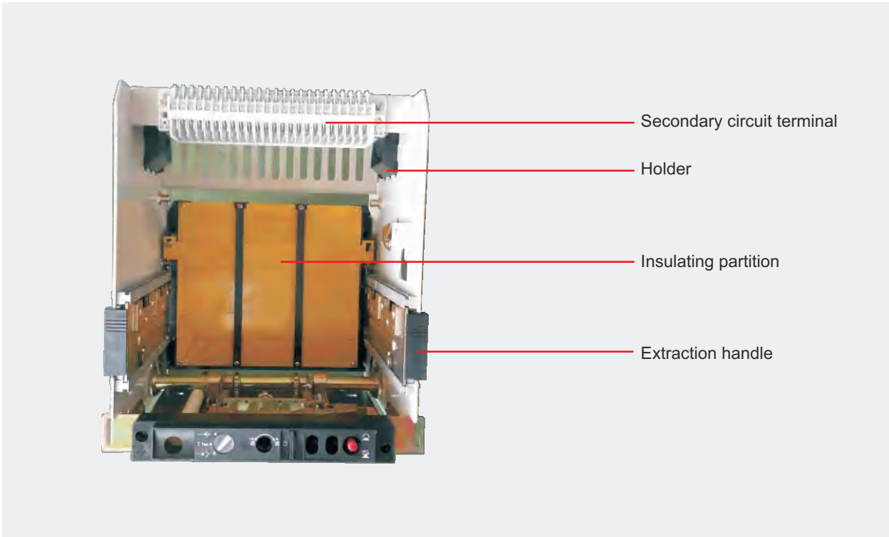
Figure 7. Drawer seat of the KNW1 Series Universal Circuit Breaker
